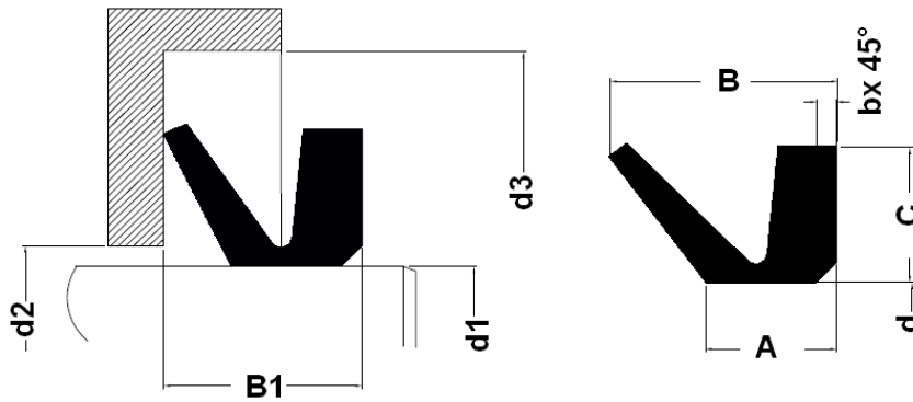
Dimension table -V-SEAL Type VL
