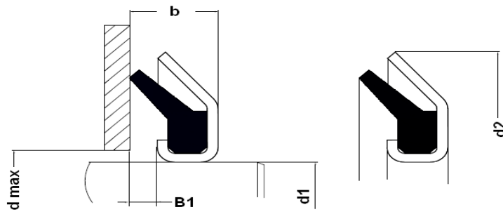
Dimension table -Gamma Seal Type RE / RB
