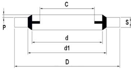
Dimension table -Bonded seal / Self Centering Type SCR
