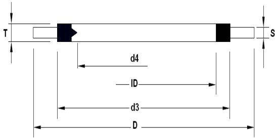
Dimension table -Bonded seal Type GM2000
